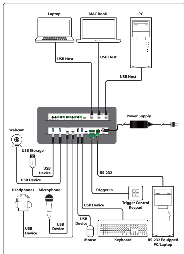
Rear View
