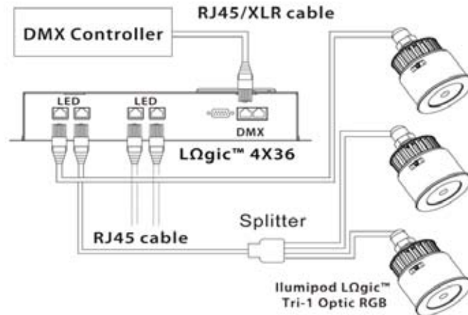
Connection Diagram
