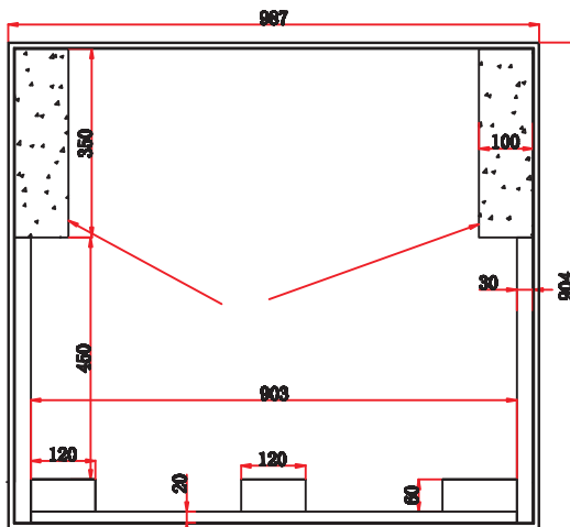
TOP VIEW OF COVER
