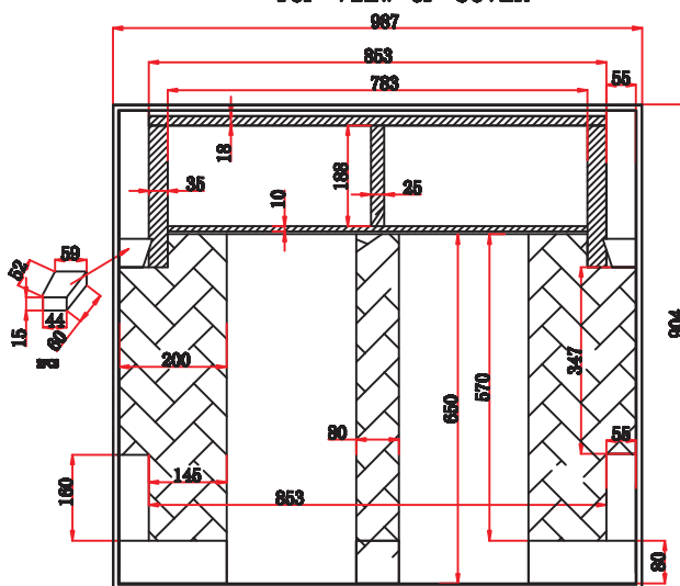
TOP VIEW OF BASE
