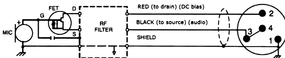
Figure 3 : Wiring diagram
