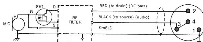
Figure 3 : Wiring diagram
