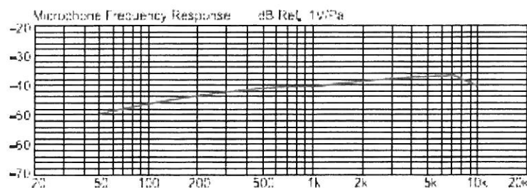
Figure 2 : Frequency response
