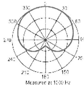
Figure 1 : Polar pattern
